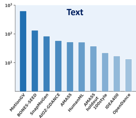
(a) Dataset Hours per Modality
